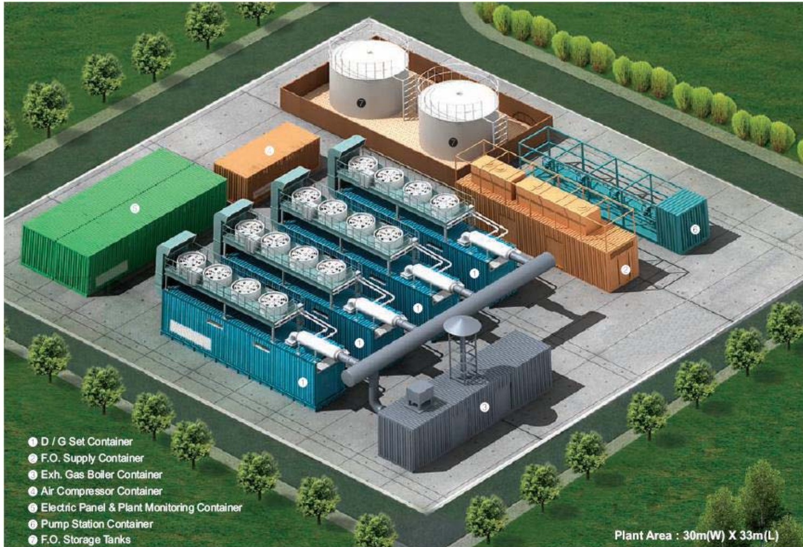
10 Megawatts Heavy Fuel Oil Power Plant Instalation
