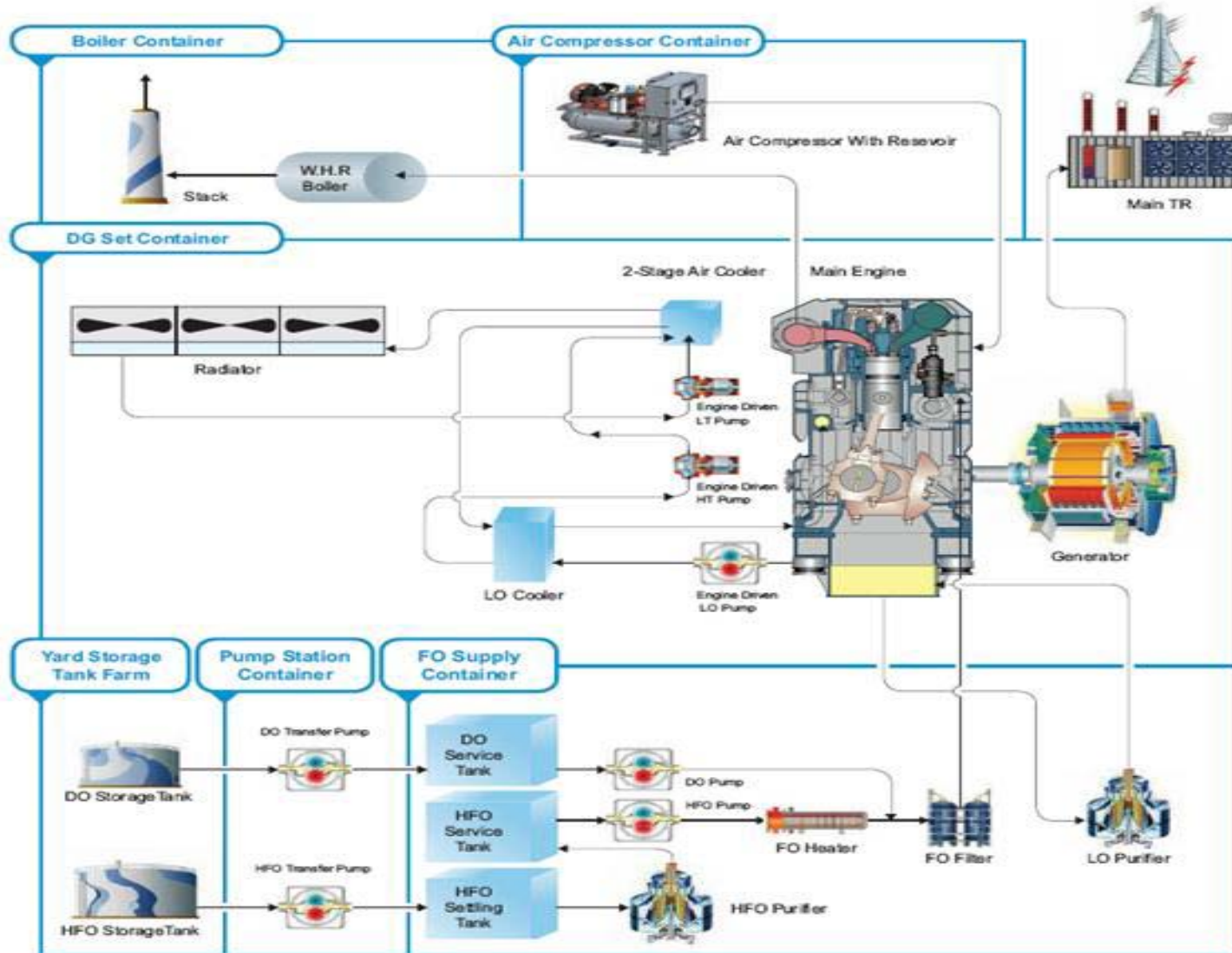
Heavy Fuel Oil Generation System Diagram
